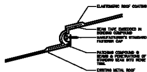
B. RIDGE FLASHING
