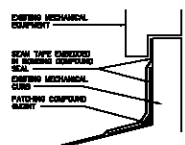
8 BASE FLASHING @ CURB A103 SCALE: 1 1/2" = 1'-0"
