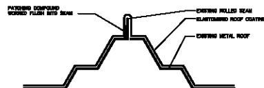
C. STANDING SEAMS
