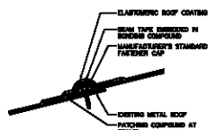
A. PANEL SEAMS
