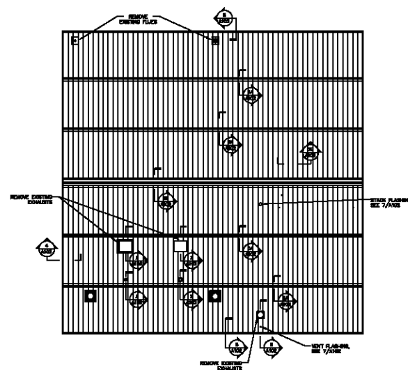
1 ROOF PLAN A103 SCALE: 1/16" = 1'-0"
