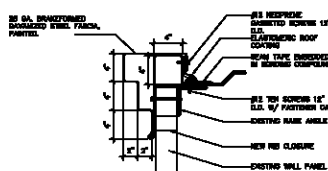
10 BASE FLASHING @ CURB A103 SCALE: 1 1/2" = 1'-0"
