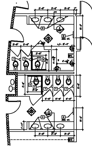
1 FIRST FLOOR RESTROOM PLAN A401 SCALE: 1/4" = 1'-0"
