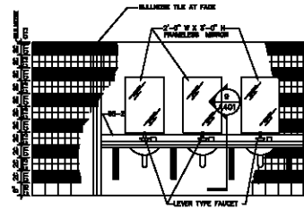
6 MEN'S RESTROOM A401 SCALE: 3/8" = 1'-0"
