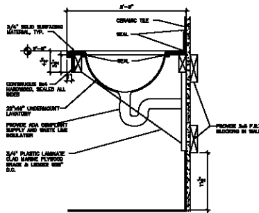
11 LAVATORY COUNTER A401 SCALE: 1 1/2" = 1'-0"
