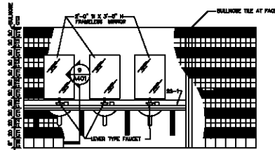
7 WOMEN'S RESTROOM A401 SCALE: 3/8" = 1'-0"
