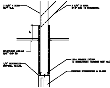
1 GYP'D BULKHEAD @ OFFICE (A31) SCALE: 1 1/2" = 1'-0"
