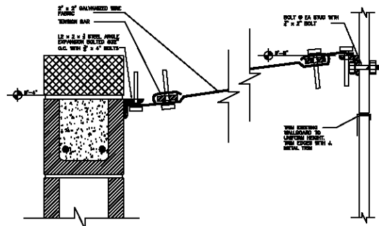
4 CHAIN LINK CLOSURE (A31) SCALE: 3" = 1'-0"
